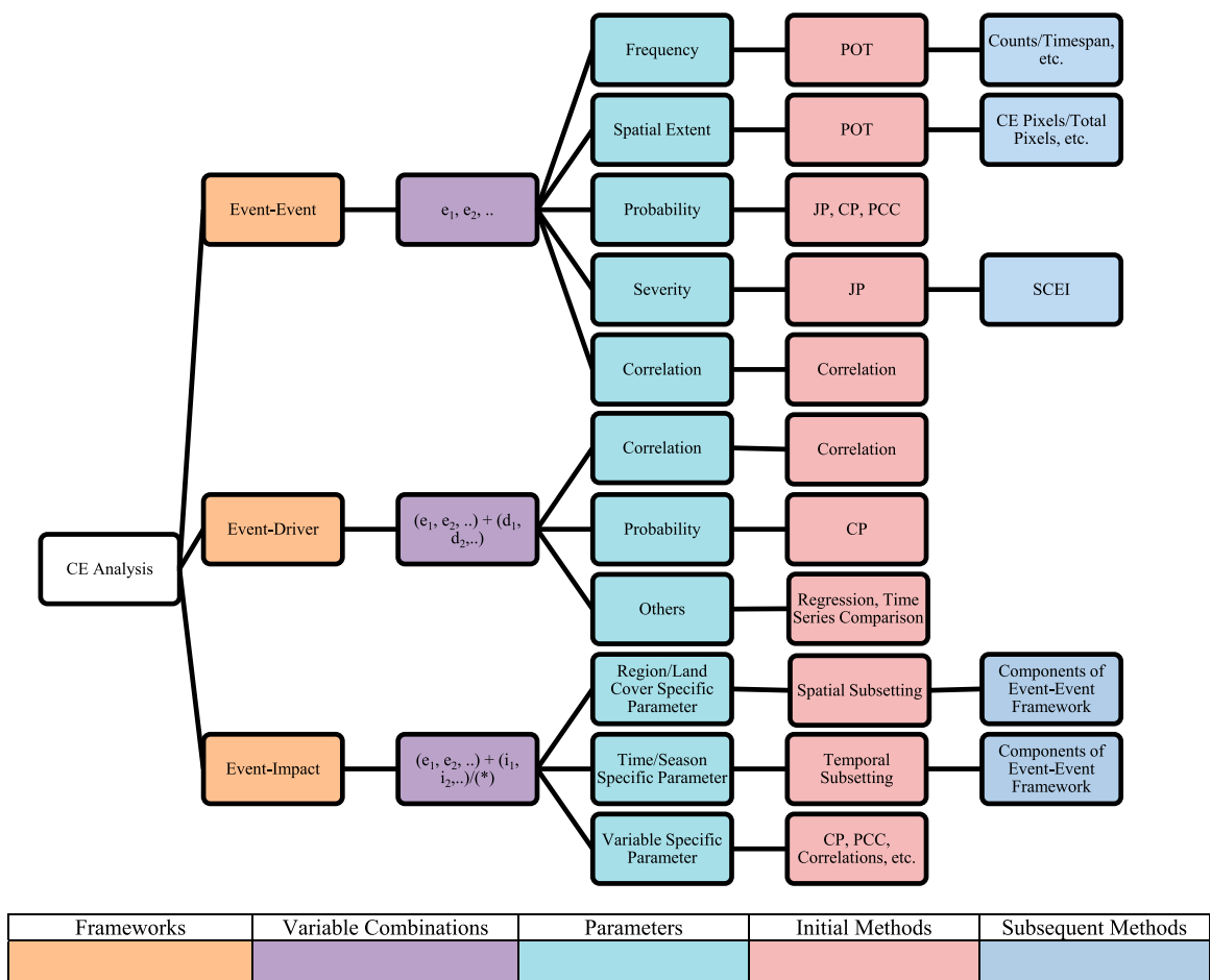
FIGURE 6 Summarized CE analysis components associated with three major analysis frameworks (event–event, event–driver, and event–impact) (here, e_n , d_n , and i_n refer to events, drivers (CVs), and impacts indicating variables/indices, respectively; (*) indicates seasonal or land use data in other forms.
